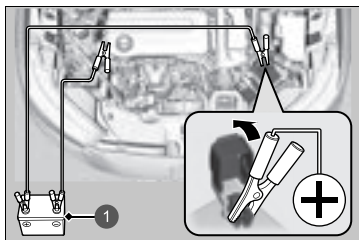
1 Booster Battery
